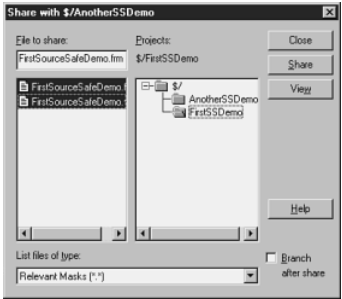
FIGURE 2.18▲ Sharing files.
